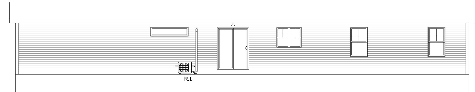
REAR ELEVATION
