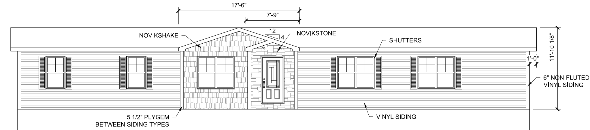
FRONT ELEVATION
